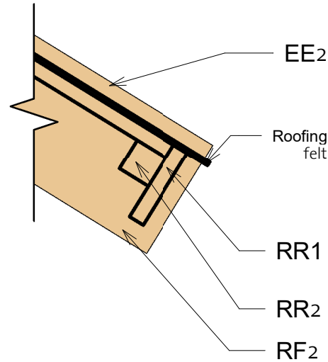
② Roof Reinforcement
